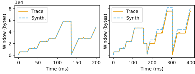
Figure 2: The dashed line shows the visible window produced by the candidate cCCA ( win\text{-}ack : CWND + AKD ; win\text{-}timeout = w_0 ), compared to the trace’s CCA ( win\text{-}ack : CWND + AKD ; win\text{-}timeout : CWND/2 ) shown by the solid line, for two traces with durations 200ms on the left and 400ms on the right.
